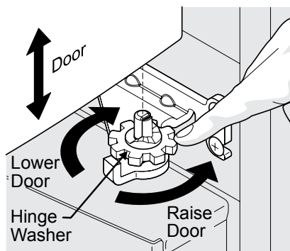
Raising/Lowering Door
