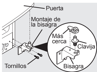
Bisagra ajustable
