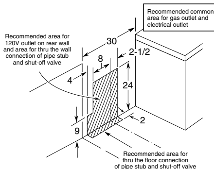
Gas Self-Clean Range Anti-Tip Bracket (Part No. 205C1714P001) JGBS23/22/20/17/10/09/07/04, JGBC20
