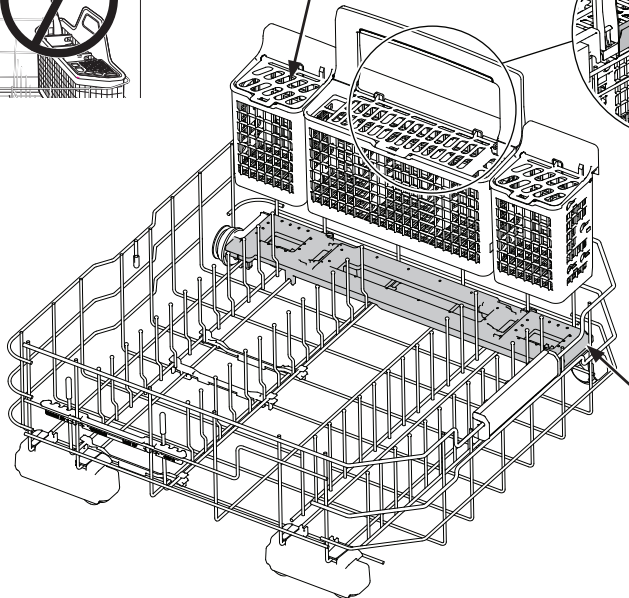
Silverware Basket - 10 Place Settings Models - GD*565, GD*645
