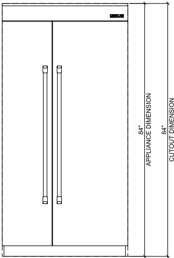
2 FRONT ELEVATION
