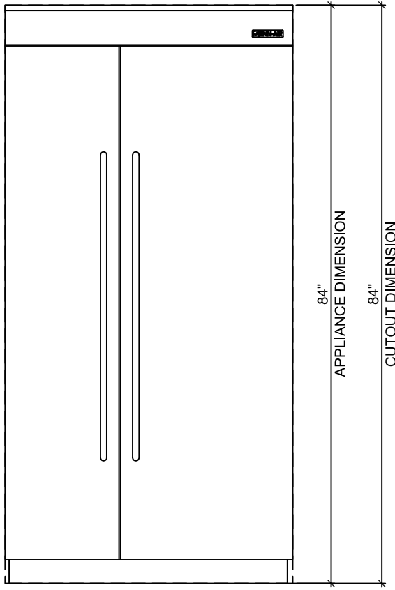
2 FRONT ELEVATION
