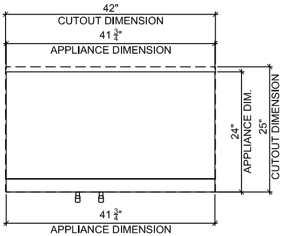
1 PLAN
