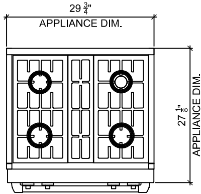
1 PLAN
