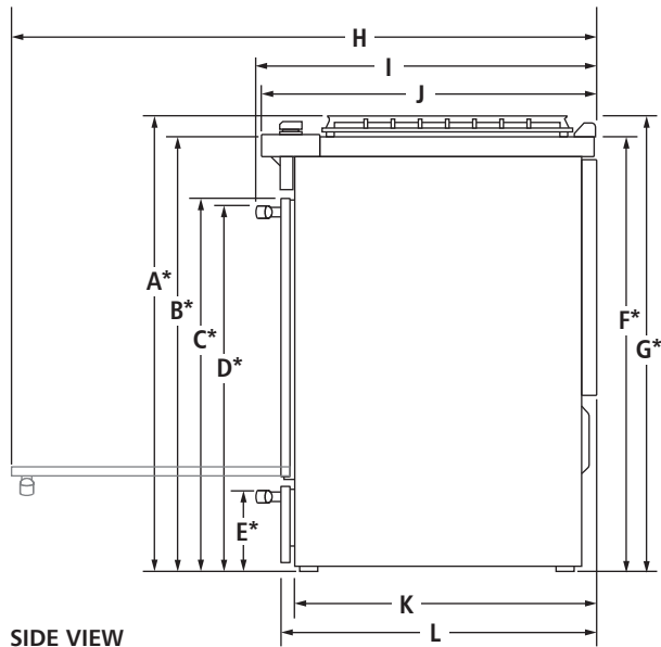
SIDE VIEW
