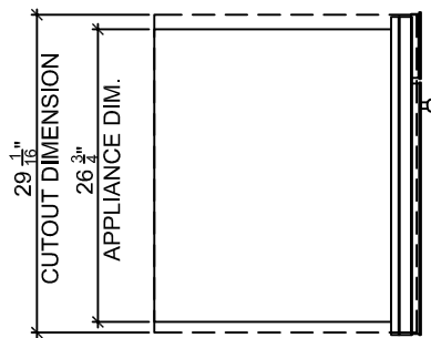
3 SIDE ELEVATION
