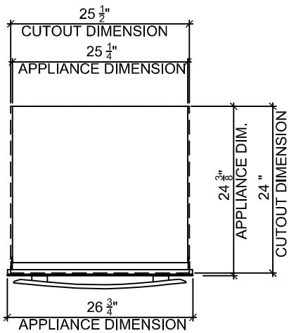
1 PLAN
