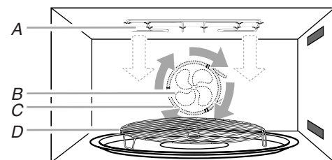
A. Broil element B. Convection fan C. Convection element D. Convection grid
