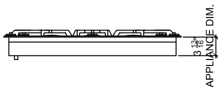
2 FRONT ELEVATION
