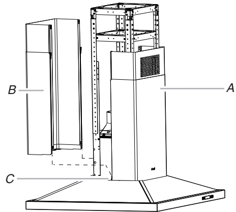
A. Duct cover (front assembly) B. Duct cover (rear assembly) C. Plastic clips (2) - in front lower duct cover.
