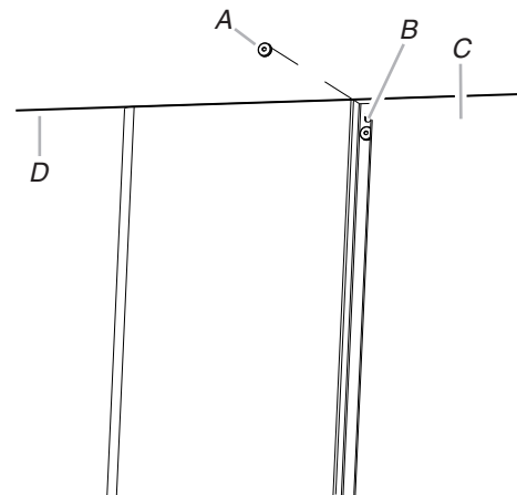
A. 3 x 6 mm Screws (2) B. Slotted holes (2) C. Upper chimney covers (assembled) D. Ceiling
