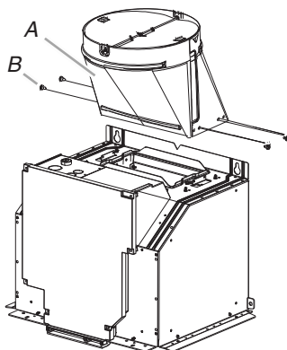
A. Vent transition B. 4 x 8 mm screws (4)
