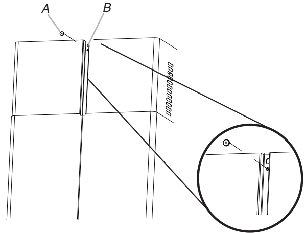
A. 3 x 6 mm screws (2) B. Assembly holes (larger hole outside the smaller hole on both sides)
