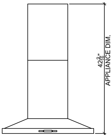
2 FRONT ELEVATION
