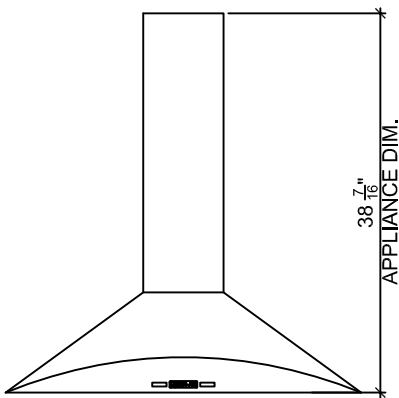
2 FRONT ELEVATION
