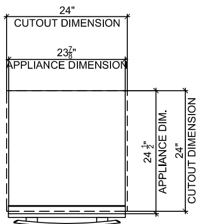
1 PLAN
