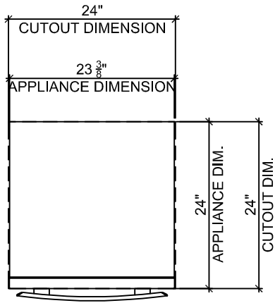
1 PLAN
