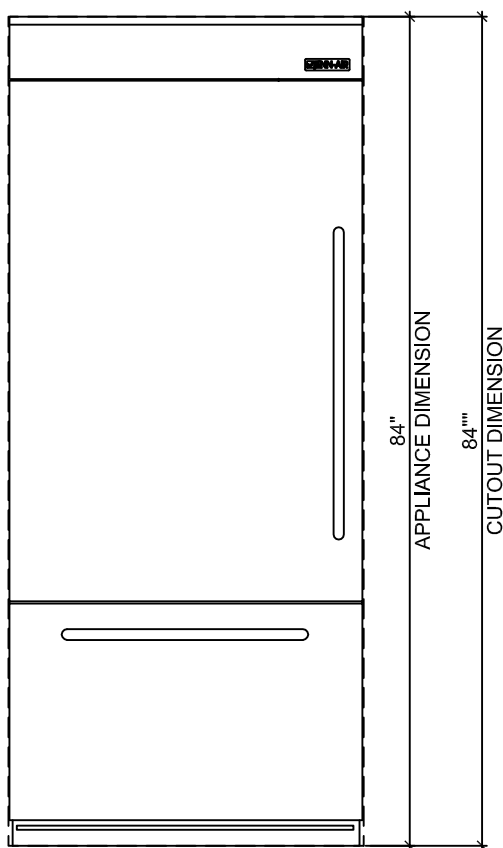
2 FRONT ELEVATION
