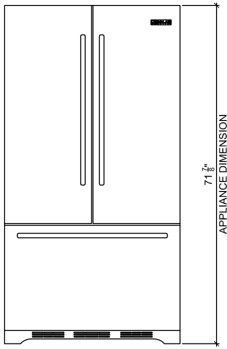
2 FRONT ELEVATION
