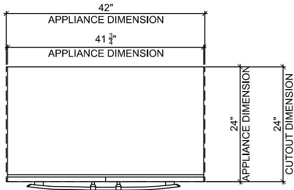
1 PLAN
