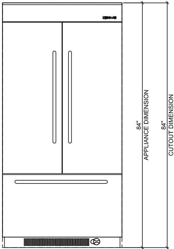
2 FRONT ELEVATION
