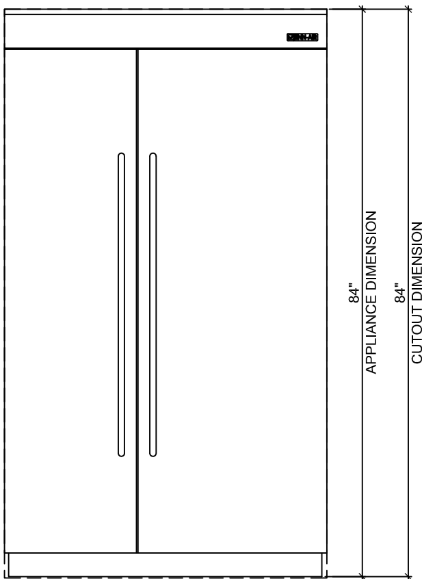
2 FRONT ELEVATION
