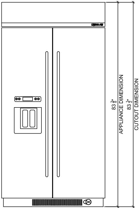
2 FRONT ELEVATION
