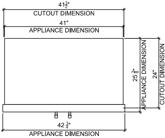
1 PLAN
