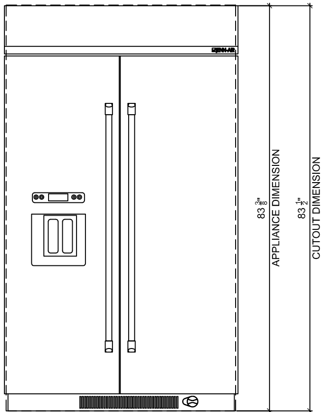
2 FRONT ELEVATION
