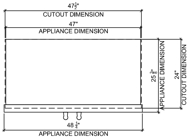
1 PLAN
