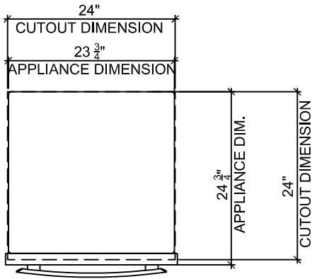
1 PLAN
