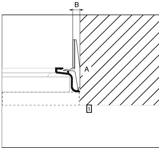
A. Lateral Connection Kit
