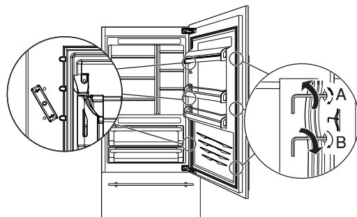
A. Shoulder Screw adjustment B. Locking Screw adjustment
