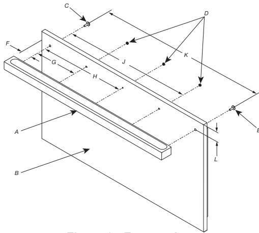
Figure 3 - Freezer drawer
