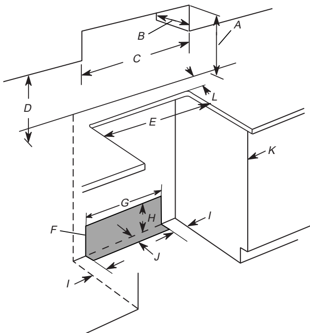
Slide-In Cutout
