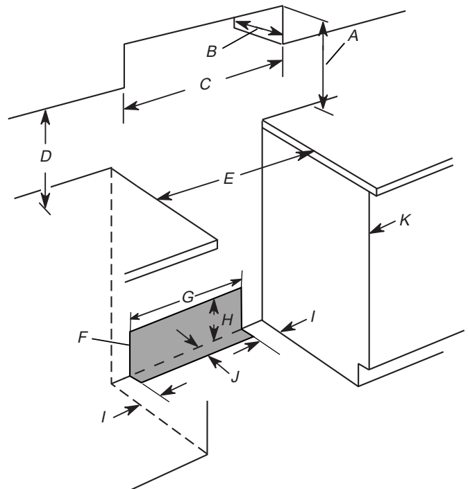
Freestanding Cutout
