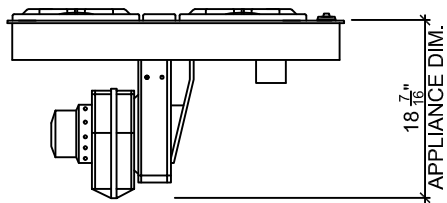
2 FRONT ELEVATION
