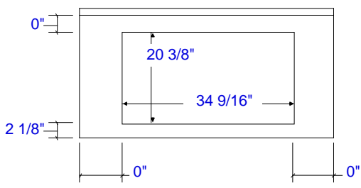
Cut-Out Dimensions Countertop View (not to scale)
