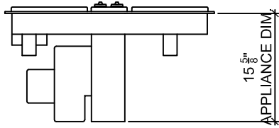
2 FRONT ELEVATION
