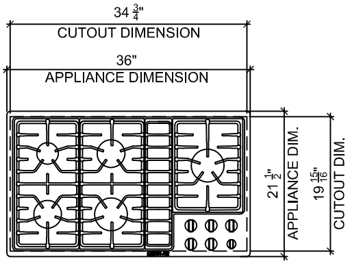
1 PLAN
