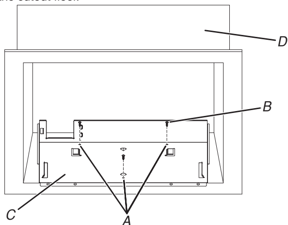
A. Bottom duct mounting holes B. 123# screws (3) C. Bottom duct D. Cabinet
