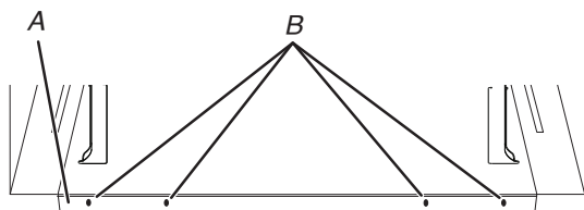
A. Bottom duct flange B. Mounting holes
