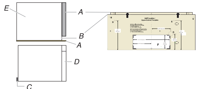
A. Front Edge of Cardboard Plate Upper Cabinet Door B. Upper Cabinet Cardboard Plate 0.75" (1.9 cm) Line C. Mounting plate D. Microwave oven door Cabinet
