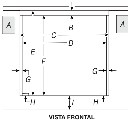
VISTA FRONTAL
