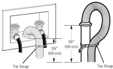
Tie Strap
