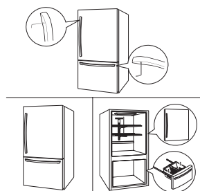
3 Disassembling/Assembling
