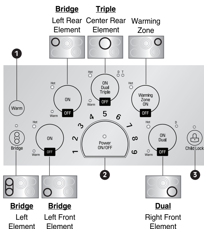
UPCE3664ST Radiant Cooktop
