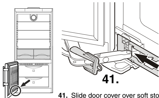
41. Slide door cover over soft stop mechanism hinge.
