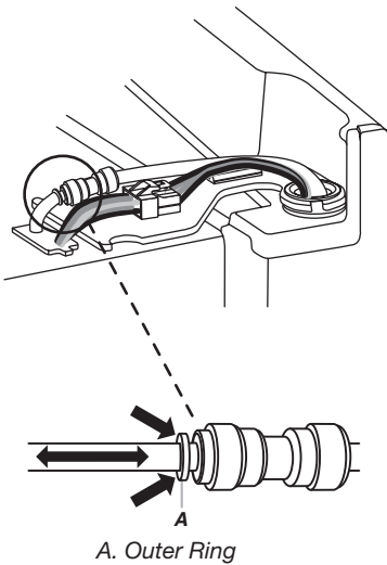
Style 1 – Water Dispenser Tubing Connection
