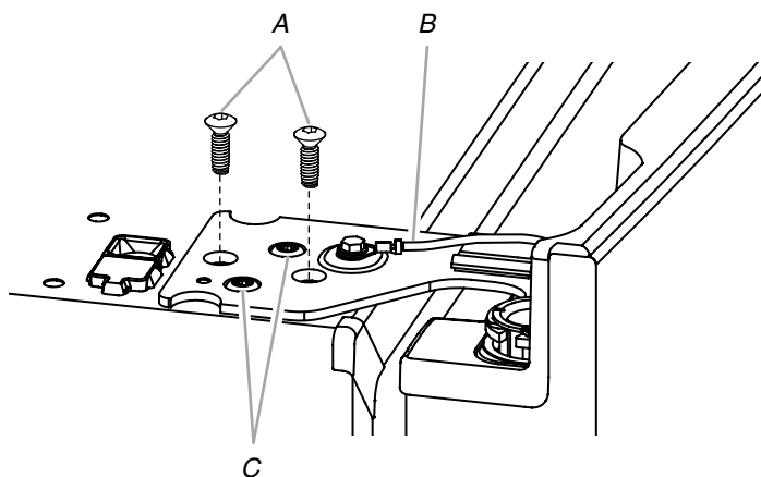
A. \frac{3}{16} " Internal hex head screws C. Locator screws (do not remove) B. Ground wire (do not remove)
