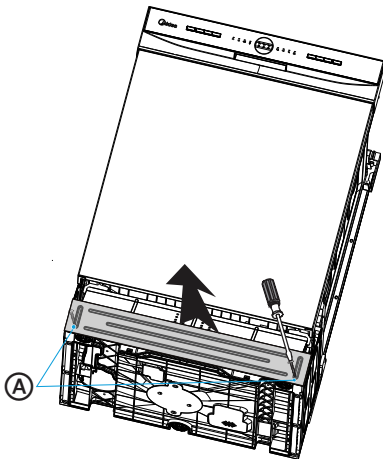
(A) Kick Plate Screws (2)
