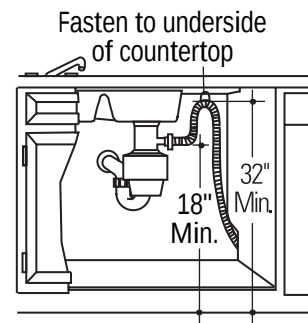
Disposer Installation
