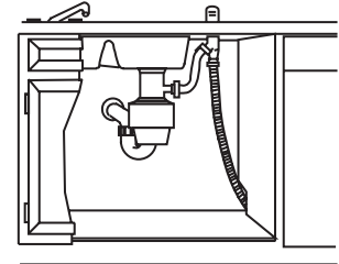
Disposer Installation
