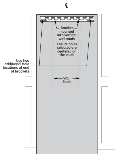
FRONT VIEW OF CUTOUT WITH ANTI-TIP BRACKET
