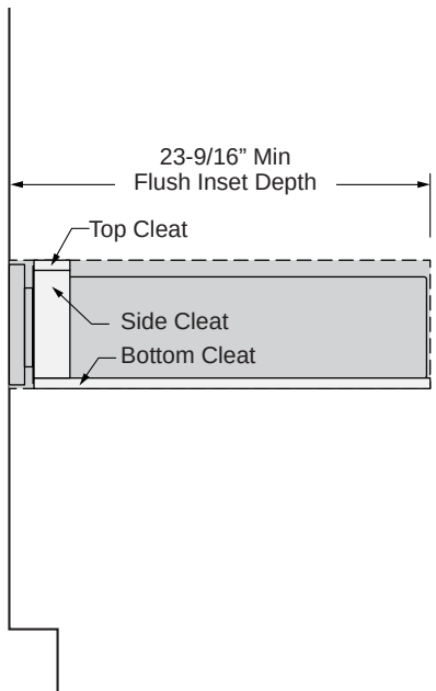
FLUSH INSET INSTALLATION SIDE VIEW
