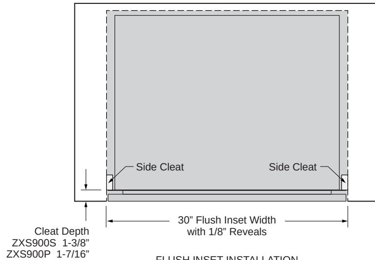
FLUSH INSET INSTALLATION TOP VIEW
