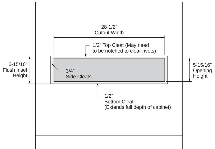
FLUSH INSET INSTALLATION FRONT VIEW
