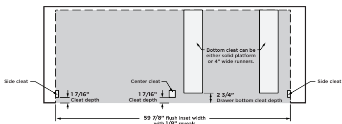
FLUSH INSET INSTALLATION TOP VIEW
