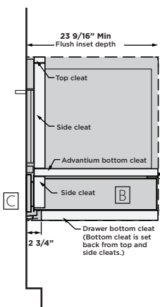
FLUSH INSET INSTALLATION SIDE VIEW
