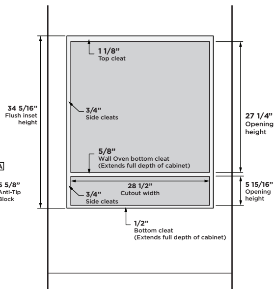
FLUSH INSET INSTALLATION FRONT VIEW
