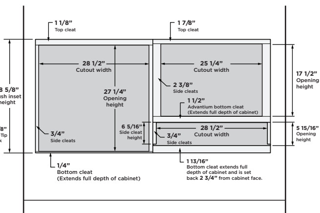
FLUSH INSET INSTALLATION FRONT VIEW
