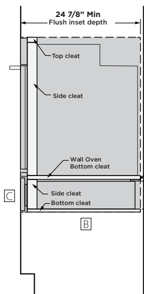
FLUSH INSET INSTALLATION SIDE VIEW
