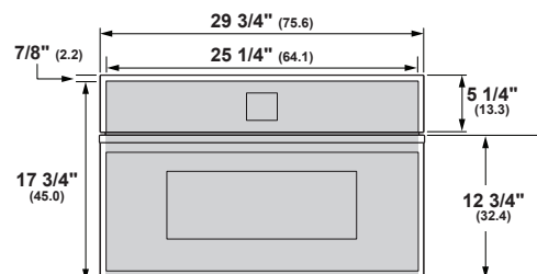
FRONT VIEW (SHOWING CUTOUT OVERLAP)
