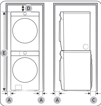
Stacked installation
