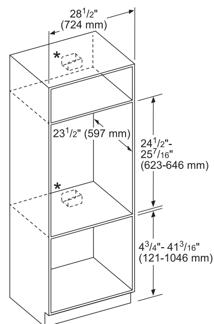
Single Steam Oven Wall mount installation
