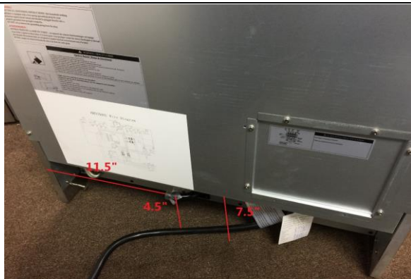
Picture of the Range's Back
