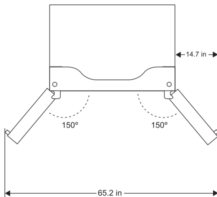
TOP OF REFRIGERATOR WITH DOORS OPEN 150°
