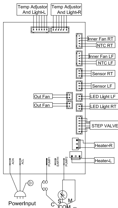
Electrocircuit Line Diagram
